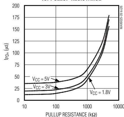
MAX9026/MAX9028 PROPAGATION DELAY ( t_{PD+} ) vs. PULLUP RESISTANCE
