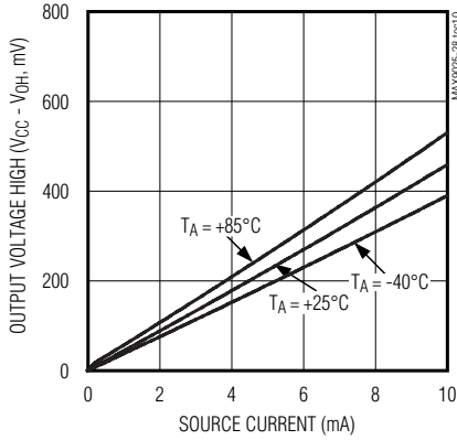
MAX9025/MAX9027 OUTPUT VOLTAGE HIGH vs. SOURCE CURRENT
