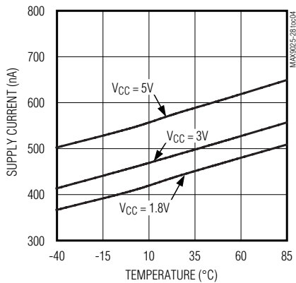
MAX9027/MAX9028 SUPPLY CURRENT vs. TEMPERATURE
