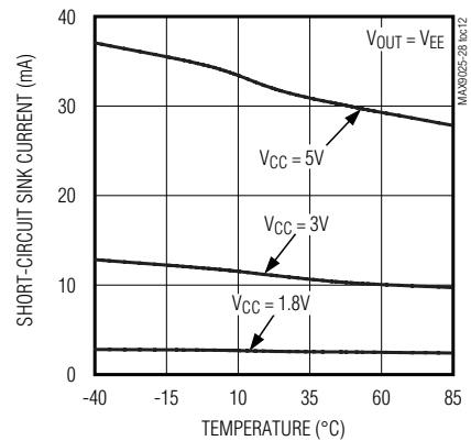
MAX9025/MAX9027 SHORT-CIRCUIT SOURCE CURRENT vs. TEMPERATURE
