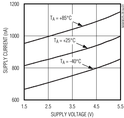
MAX9025/MAX9026 SUPPLY CURRENT vs. SUPPLY VOLTAGE
