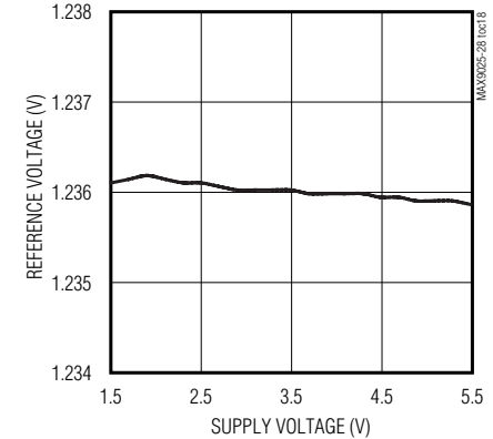
MAX9025/MAX9026 REFERENCE VOLTAGE vs. SUPPLY VOLTAGE
