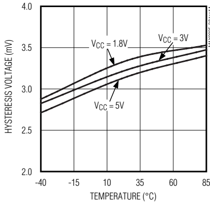
HYSTERESIS VOLTAGE vs. TEMPERATURE
