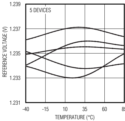
MAX9025/MAX9026 REFERENCE VOLTAGE vs. TEMPERATURE
