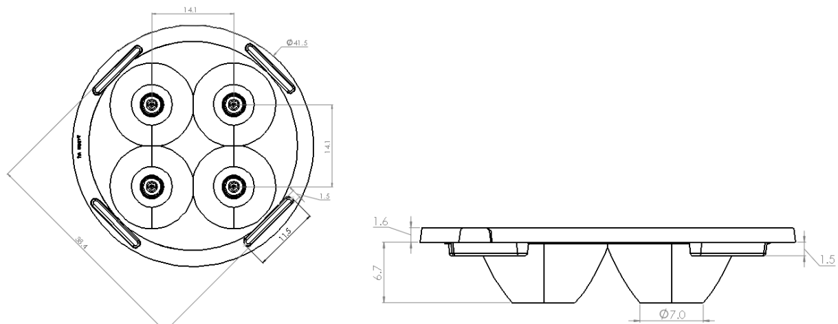
Figure 1: FD4 layout and dimensions
