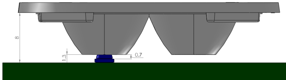
Figure 2: Optimal performance is realized when the FD4 is positioned 0.7mm above the LED package or 1.3mm (nominal) above the PCB plane.
