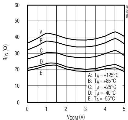
ON-RESISTANCE vs. COM VOLTAGE OVER TEMPERATURE
