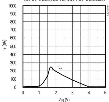
INPUT VOLTAGE vs. SUPPLY CURRENT
