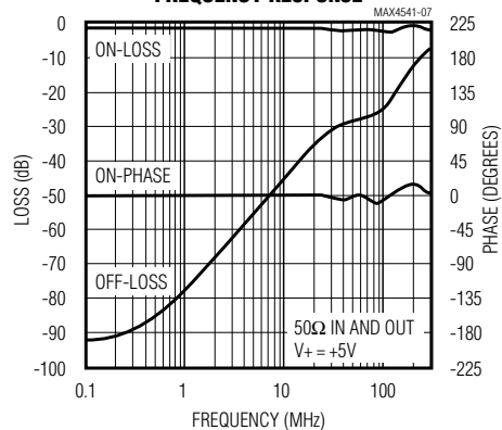
FREQUENCY RESPONSE
