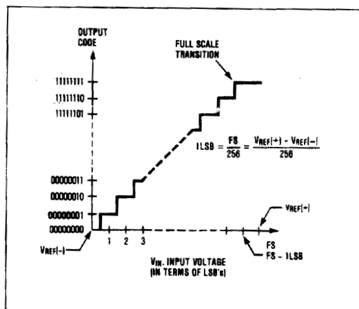
Figure 6. Transfer Function
