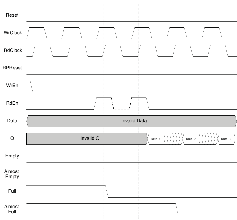
Figure 11-38. FIFO_DC with Output Registers and RdEn on Output Registers
