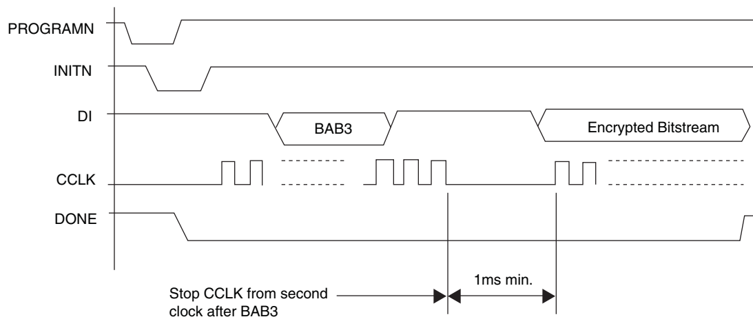
Figure 16-2. CCLK Timing
