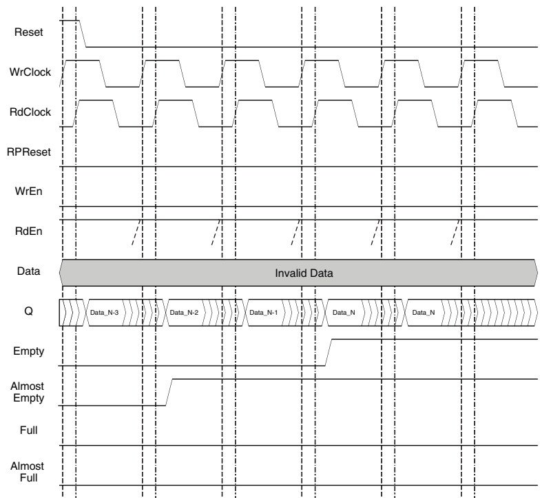
Figure 11-33. FIFO_DC without Output Registers, End of Data Read Cycle
