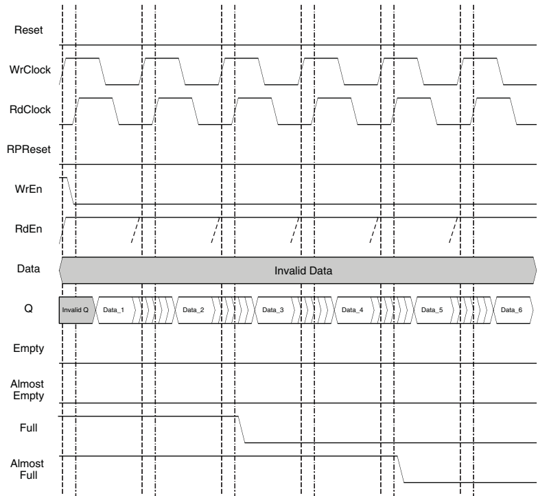
Figure 11-32. FIFO_DC without Output Registers, Start of Data Read Cycle
