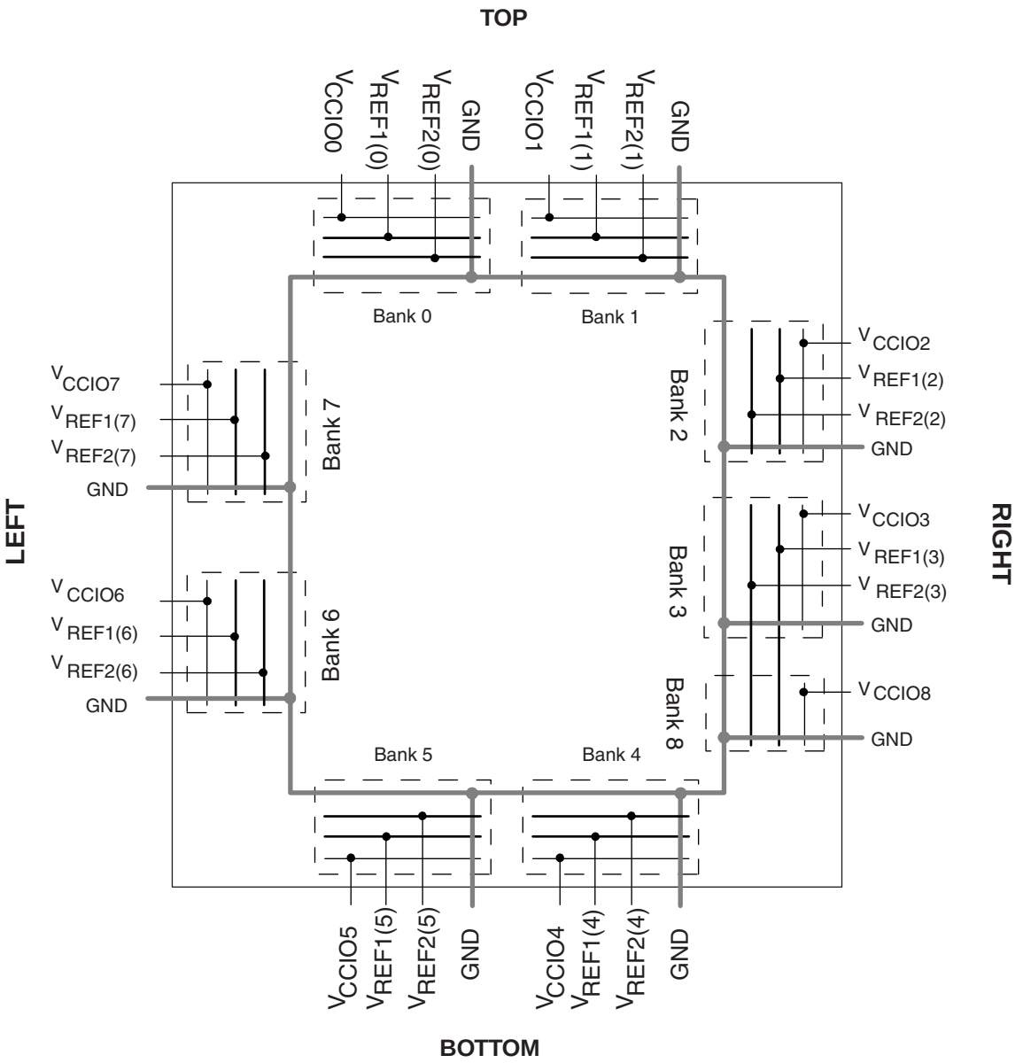
Figure 2-37. LatticeECP2 Banks
