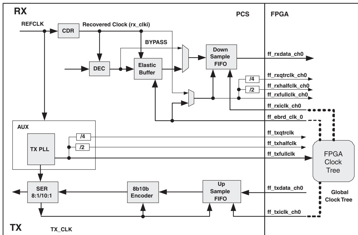
Figure 8-33. 8b10b, EB and DS FIFOs NOT Bypassed
