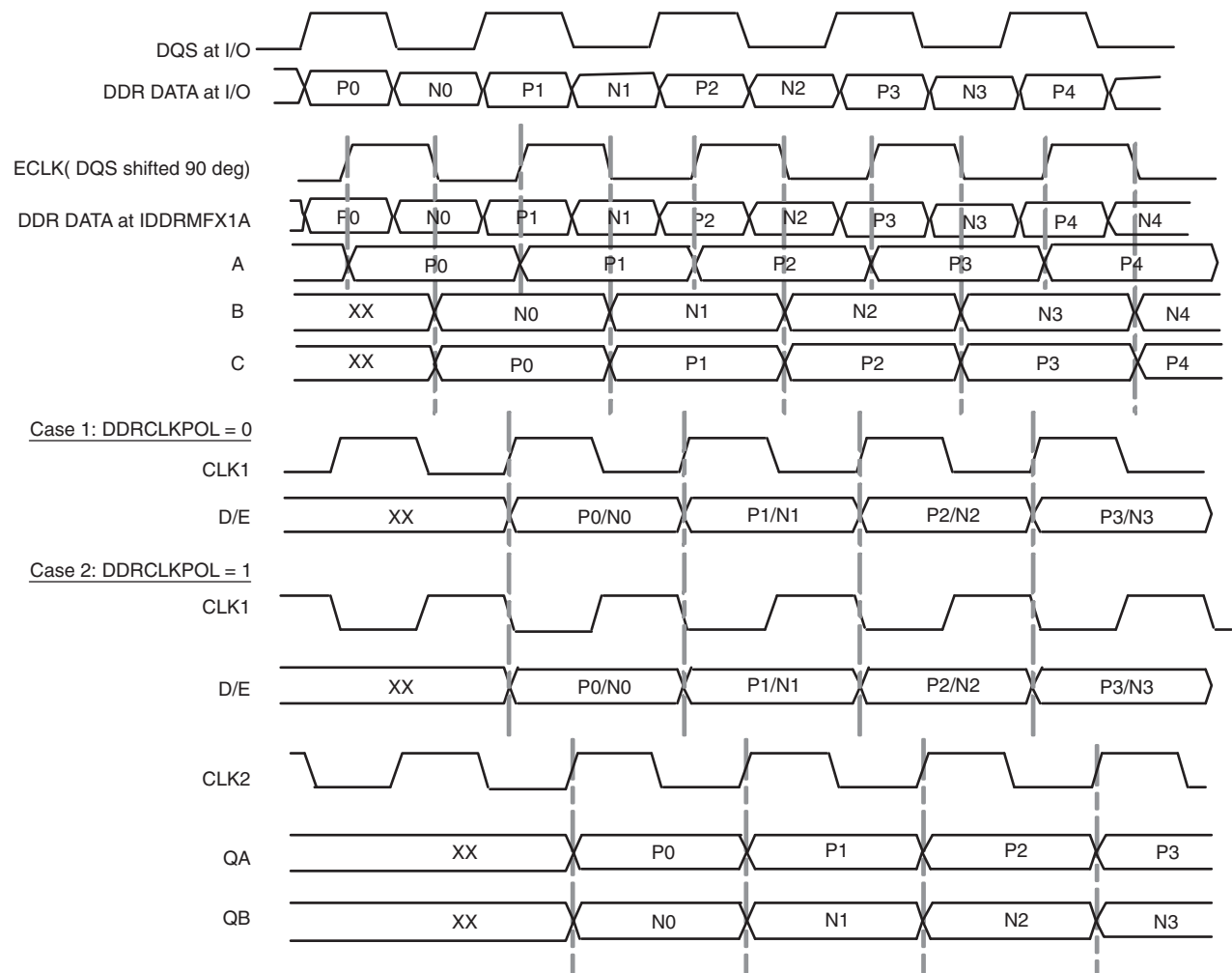
Figure 12-15. IDDRMFX1A Waveform
