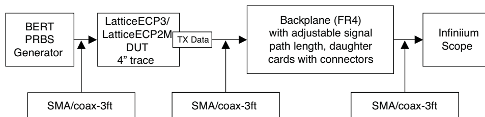
Figure 19-1. Eye Diagram Experiment Setup
