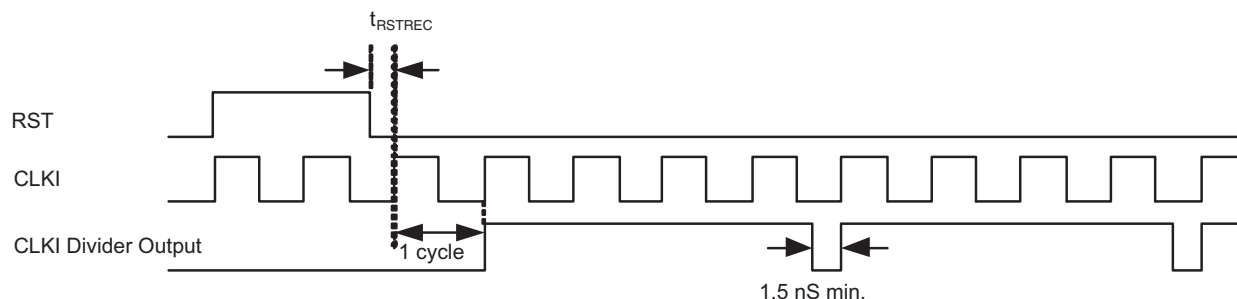
Figure 10-8. RST Input and CLKI Divider Output Timing Diagram (Example: CLKI_DIV = 4)
