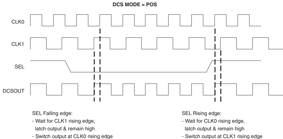
Figure 10-28. Timing Diagrams by DCS MODE
