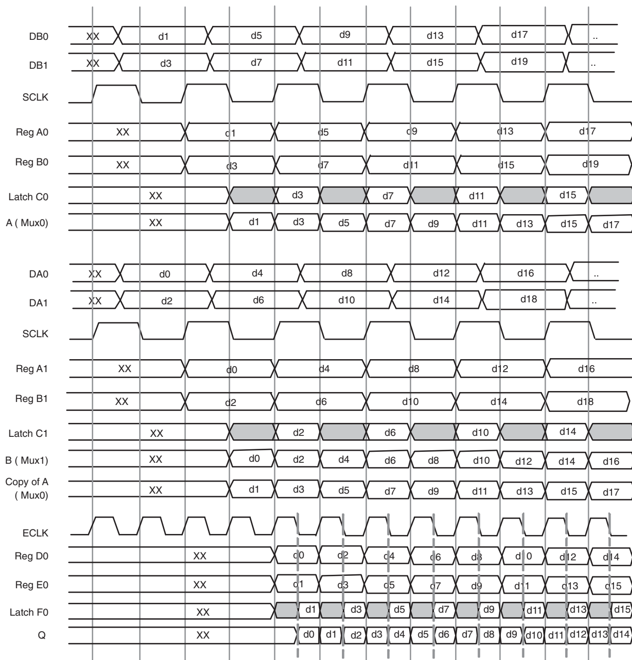
Figure 12-40. ODDRX2B Waveform
