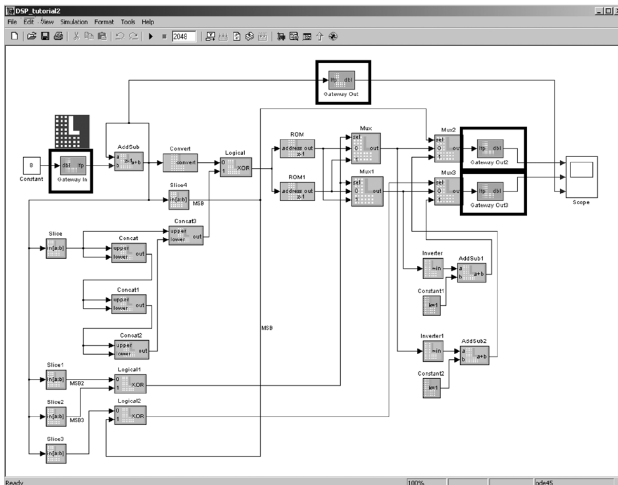
Figure 14-13. Simulink Design
