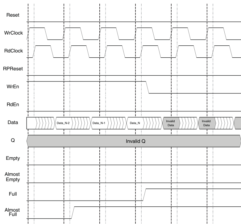
Figure 11-35. FIFO_DC with Output Registers, End of Data Write Cycle
