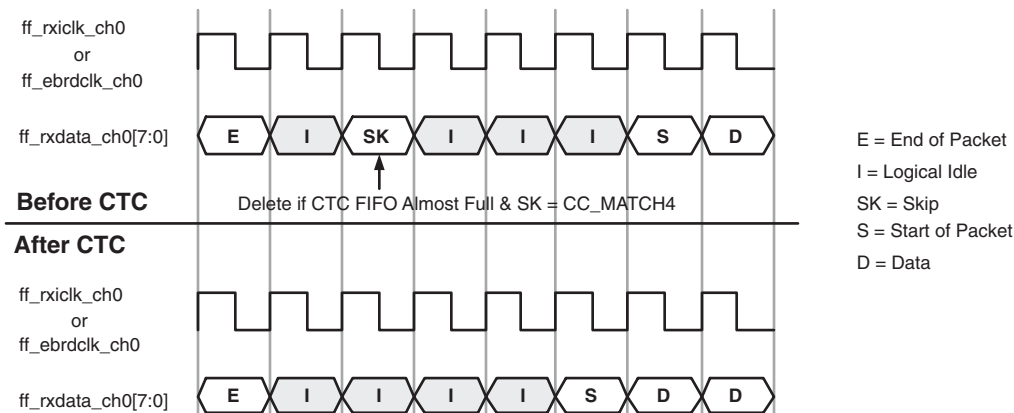
Figure 8-9. Clock Tolerance Compensation 1 Byte Deletion Example
