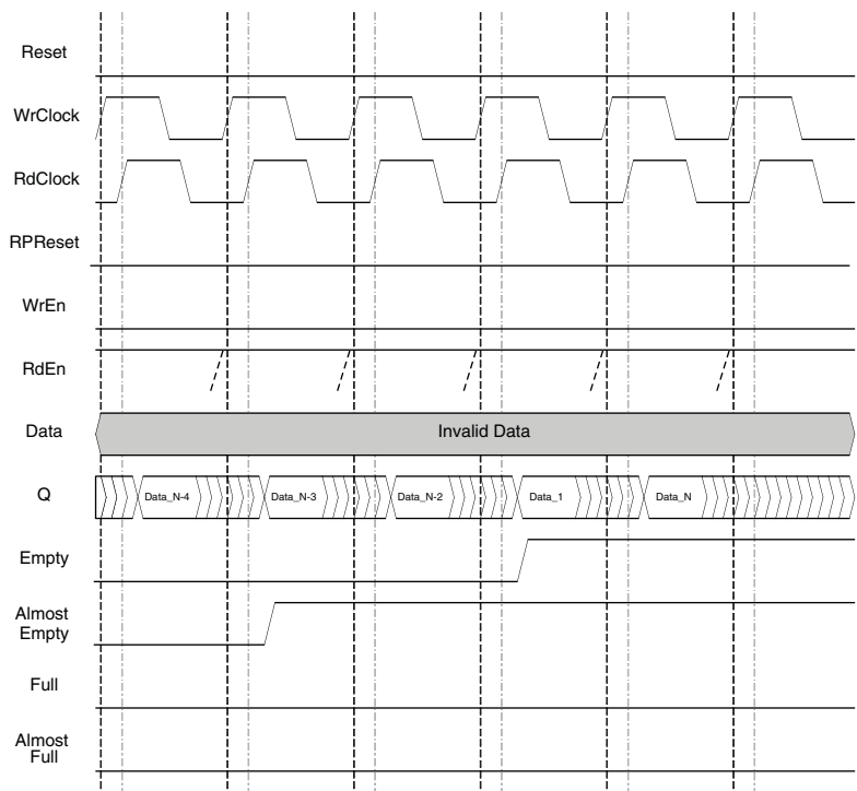
Figure 11-37. FIFO_DC with Output Registers, End of Data Read Cycle
