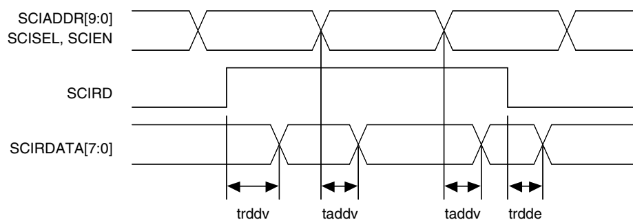
Figure 8-40. SCI READ Cycle, Critical Timing
