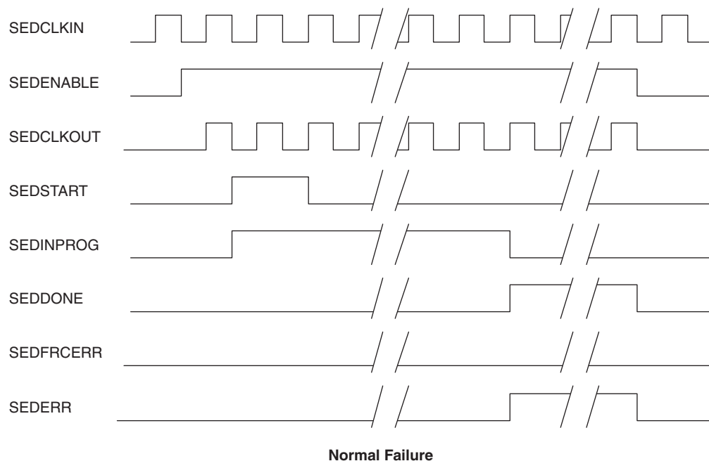
Figure 17-3. Timing Diagram
