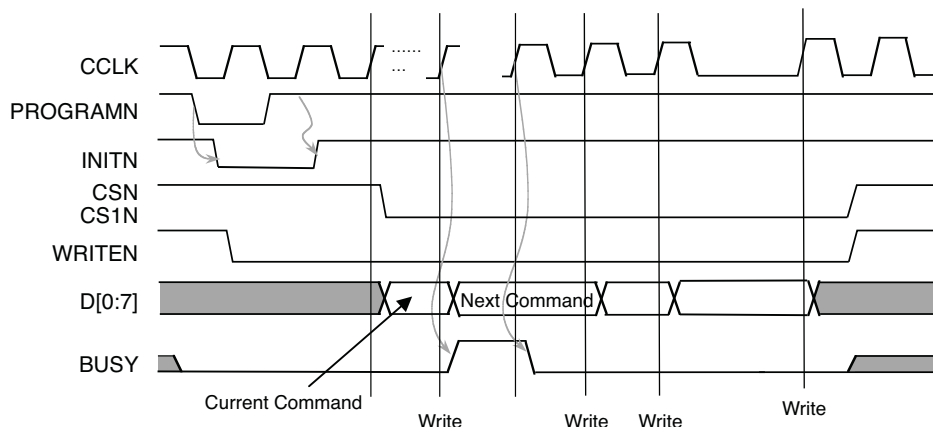
Figure 15-11. Parallel Port Write Timing Diagram
