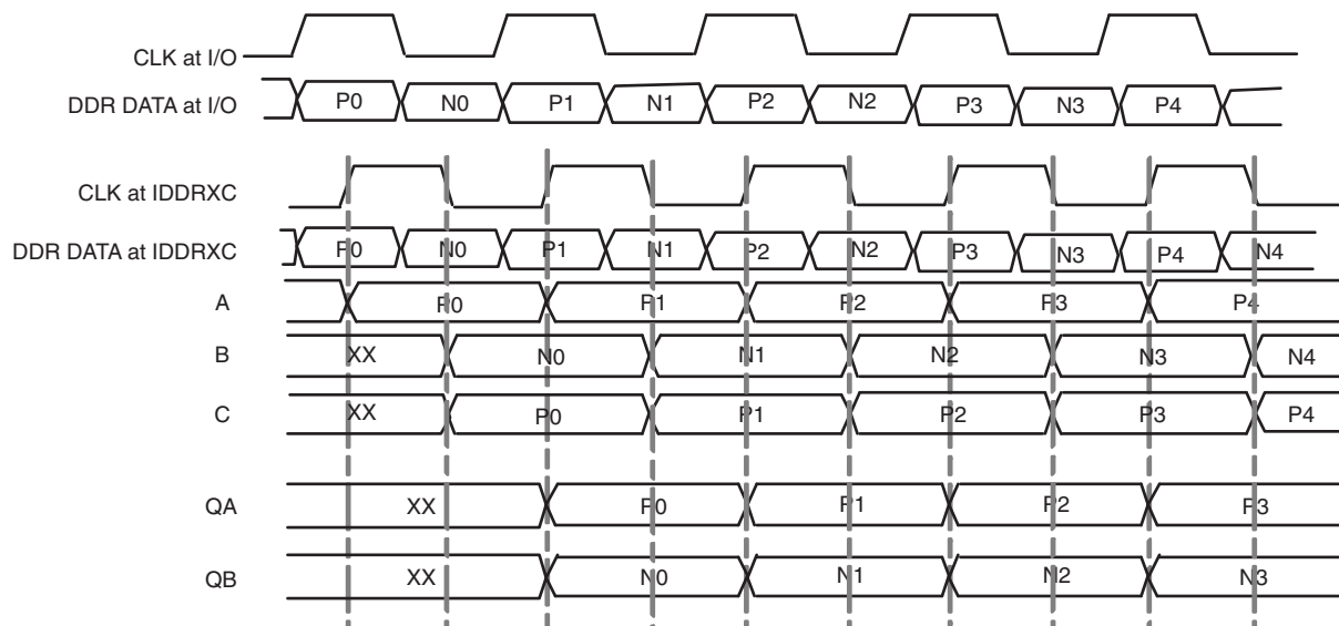
Figure 12-28. IDDRXC Waveform
