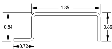
Combination Rails
