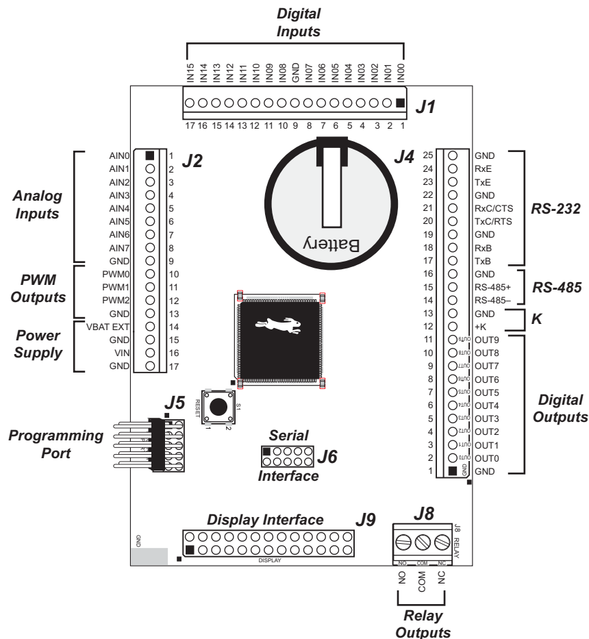
Figure 8. LP3500 Pinouts
