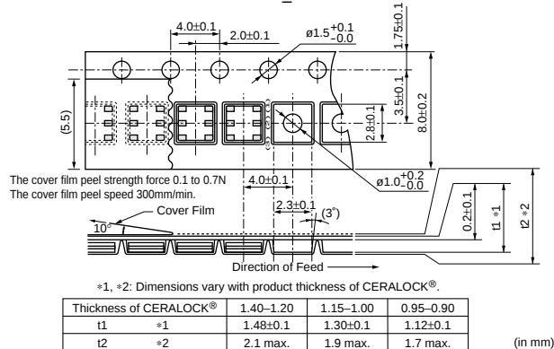
CSTCW_X11
