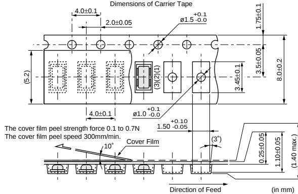
CSTCE_V_C
