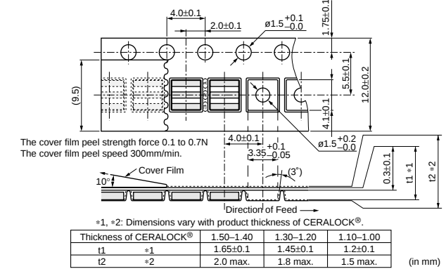
CSTCV_X_Q
