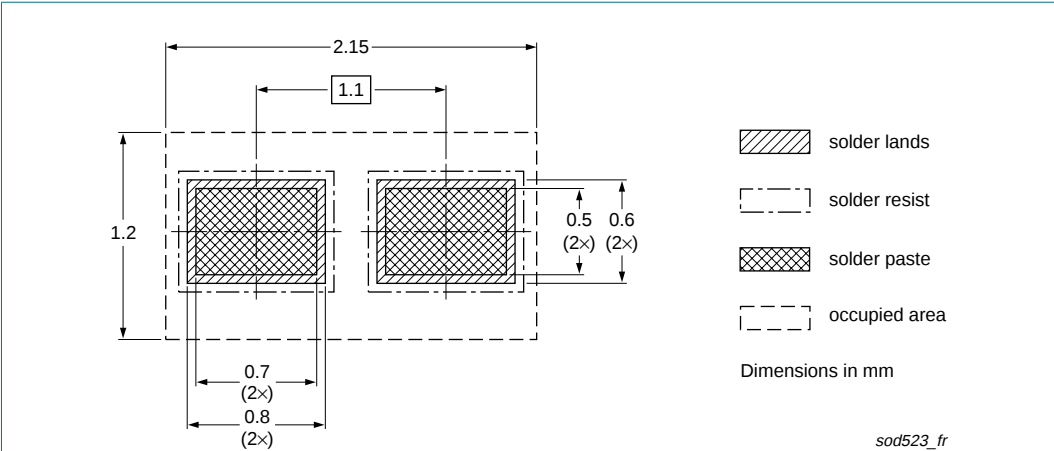
Fig 11. Reflow soldering footprint PESD5V0U1UB (SOD523/SC-79)
