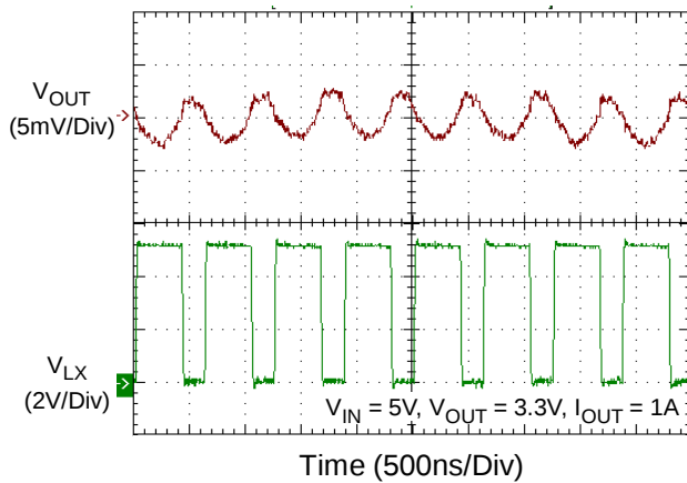
Voltage Ripple
