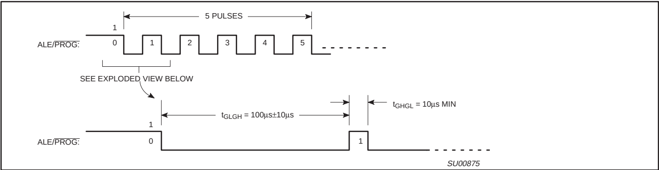
Figure 41. \overline{\text{PROG}} Waveform
