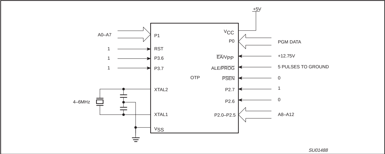
Figure 40. Programming Configuration
