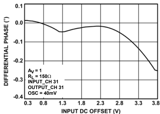
FIGURE 32. DIFFERENTIAL PHASE, A_V = 1
