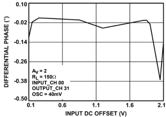
FIGURE 36. DIFFERENTIAL PHASE, A_V = 2
