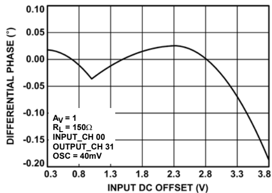
FIGURE 40. DIFFERENTIAL PHASE, A_V = 1
