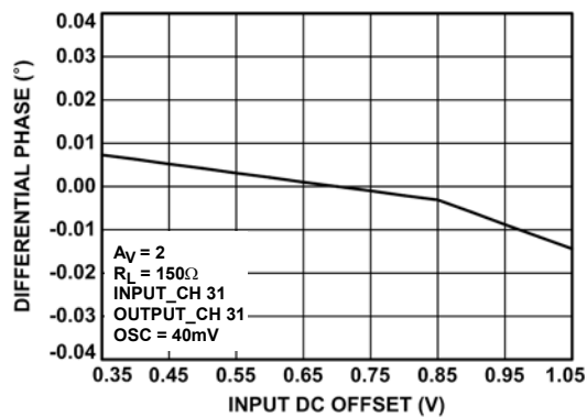
FIGURE 30. DIFFERENTIAL PHASE, A_V = 2
