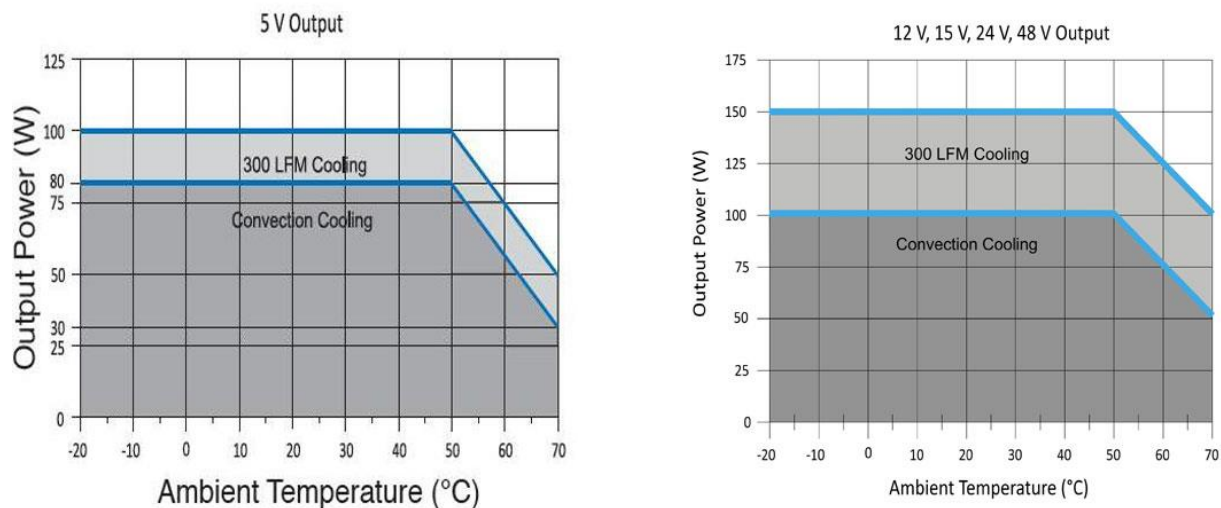
Figure 1 - Output Power Vs. Temperature
