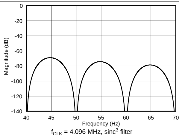
Figure 71. \text{Sinc}^3 Filter Frequency Response, Data Rate = 10 SPS, Zoomed to 50 Hz and 60 Hz
