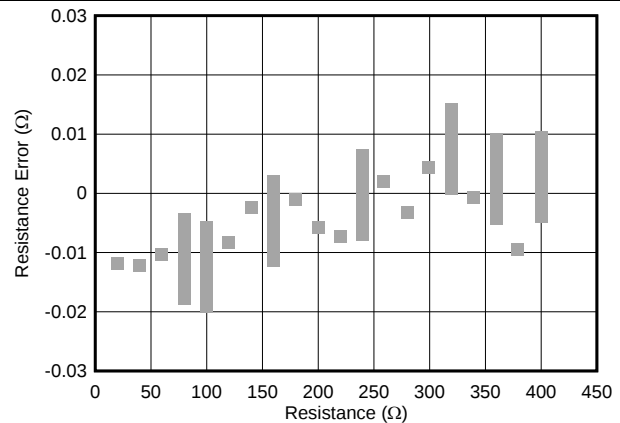
Figure 115. Measured Resistance Error vs Equivalent RTD Resistance
