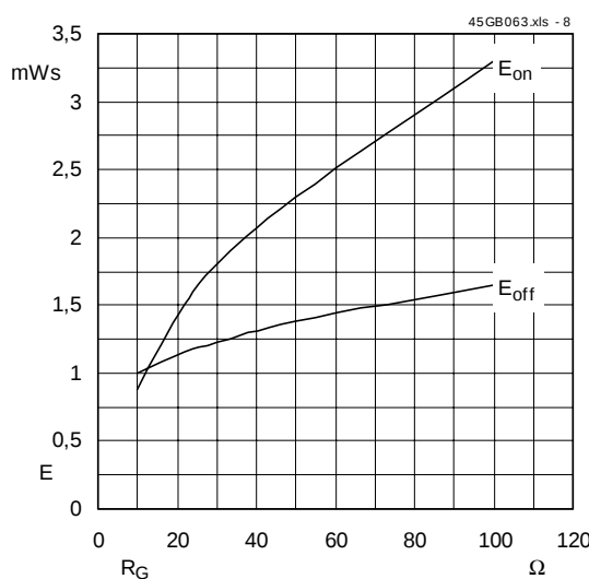
Fig. 8 Turn-on /-off energy = f(R_G)
