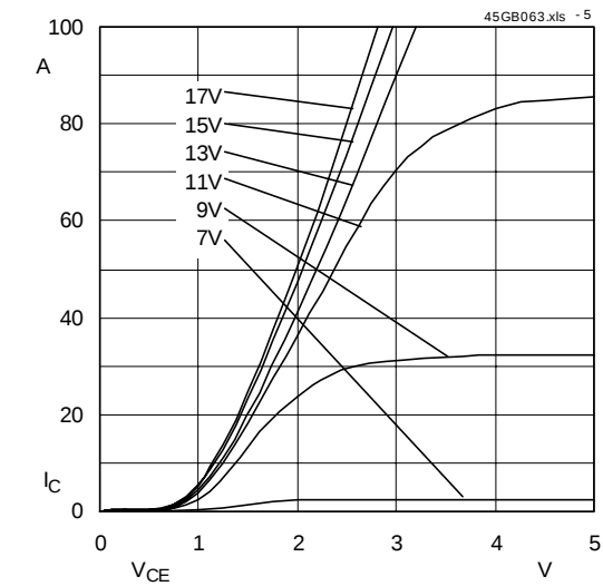
Fig. 5 Typ. output characteristic, t_p = 80 \mu s ; 25^\circ C
