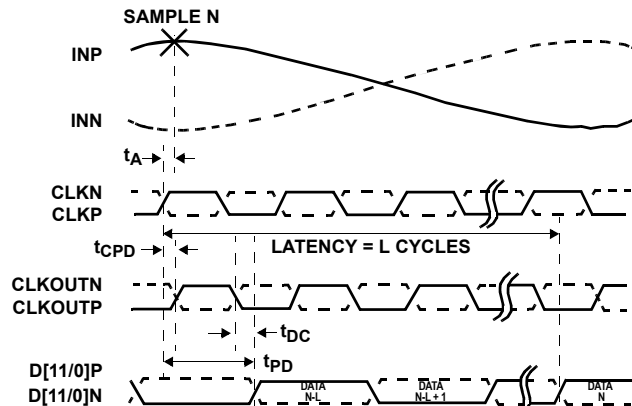
FIGURE 3B. SDR
