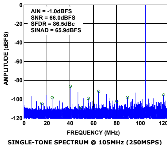
SINGLE-TONE SPECTRUM @ 105MHz (250MSPS)
