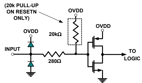
FIGURE 46. DIGITAL INPUTS
