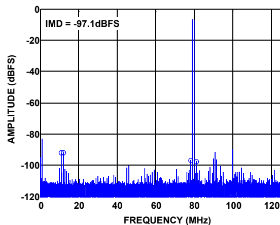
FIGURE 22. TWO-TONE SPECTRUM @ 170MHz
