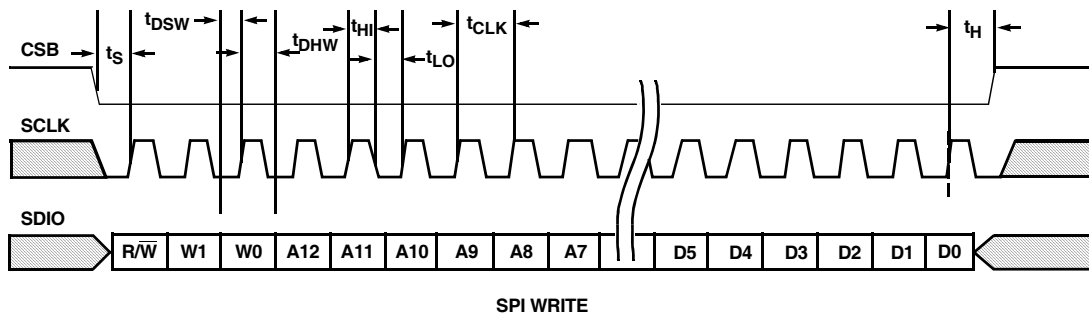
FIGURE 37. SPI WRITE
