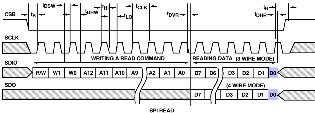
FIGURE 38. SPI READ
