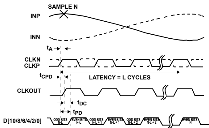
FIGURE 4A. DDR
