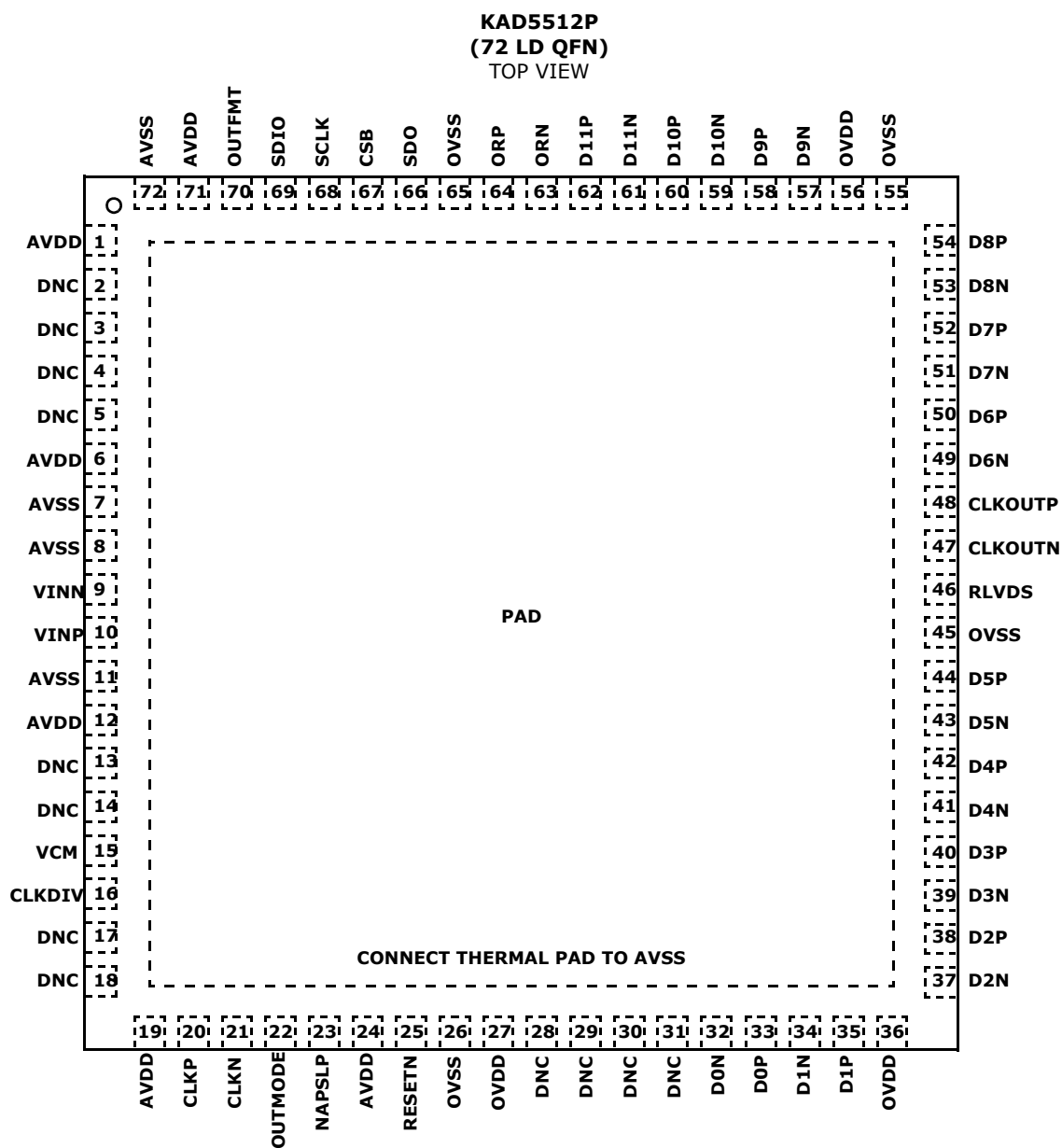
FIGURE 1. PIN CONFIGURATION
