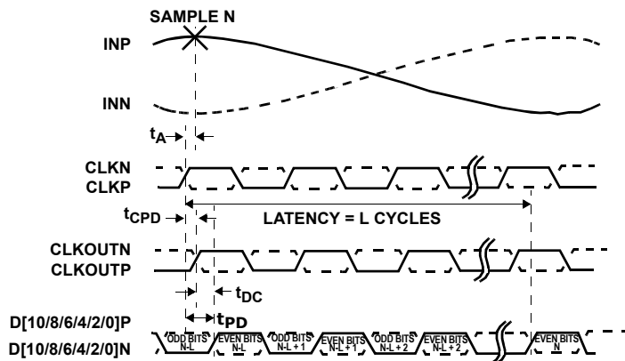
FIGURE 3A. DDR
