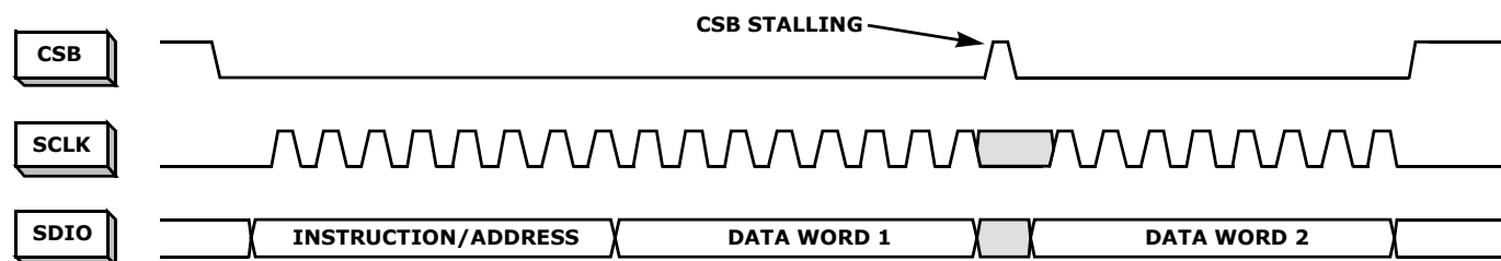
FIGURE 39. 2-BYTE TRANSFER
