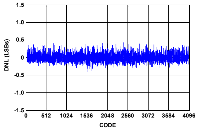
FIGURE 12. DIFFERENTIAL NONLINEARITY
