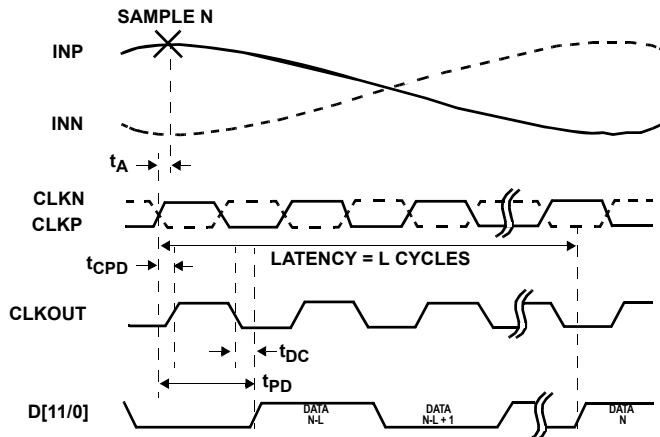
FIGURE 4B. SDR
