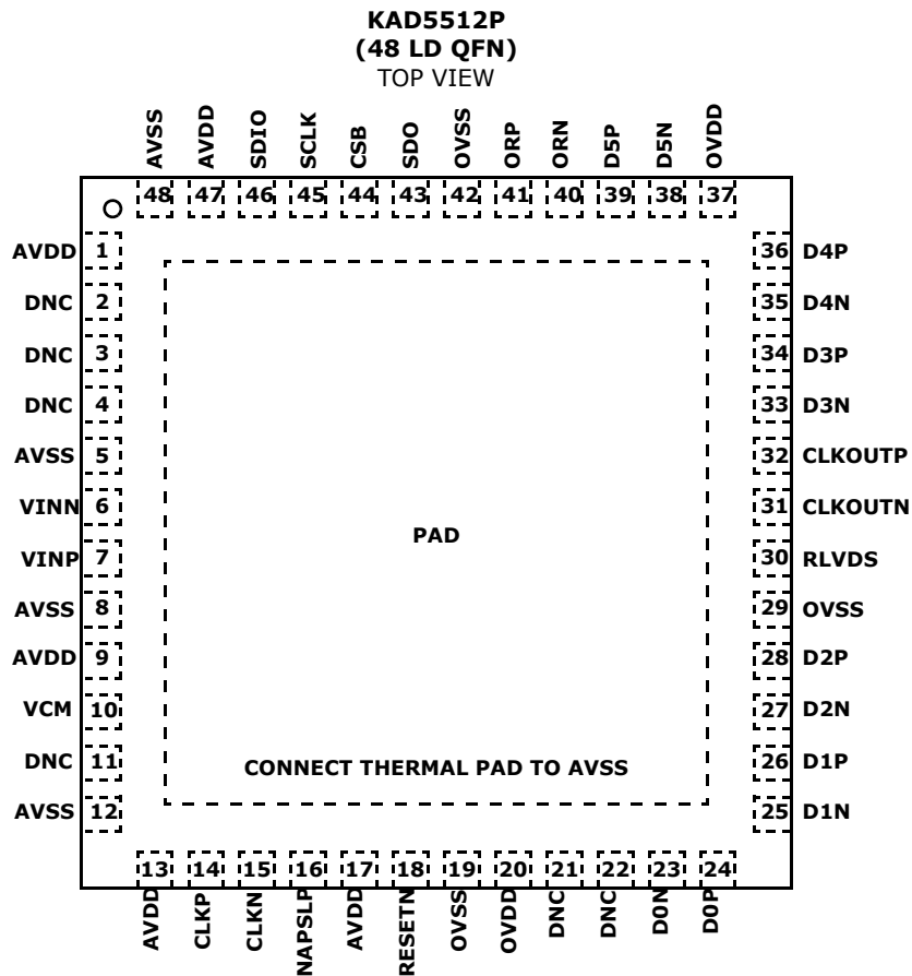
FIGURE 2. PIN CONFIGURATION
