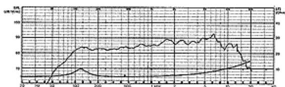
frequency- and impedance response
