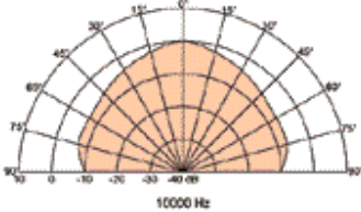
radiation pattern 10000 Hz
