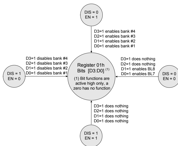
Figure 19 — Multi-function Bits of Register (01h)
