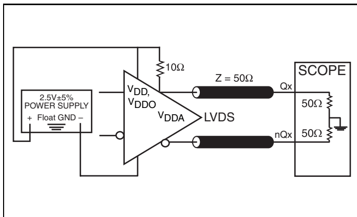
2.5V Output Load AC Test Circuit
