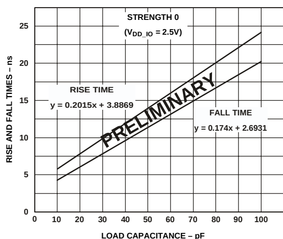
Figure 34. Typical Output Rise and Fall Time (10%–90%, V_{DD\_IO} = 2.5\text{ V} ) vs. Load Capacitance at Strength 0
