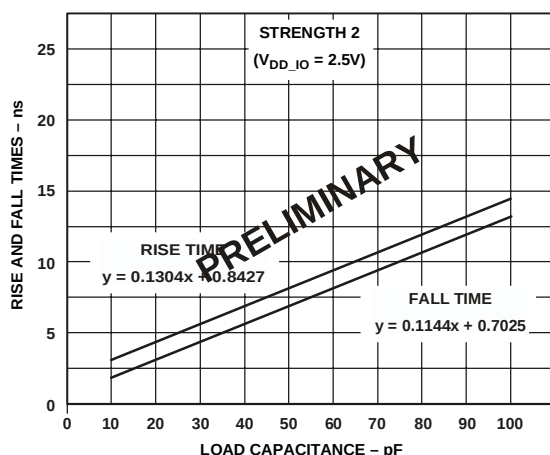
Figure 36. Typical Output Rise and Fall Time (10%–90%, V_{DD\_IO} = 2.5\text{ V} ) vs. Load Capacitance at Strength 2
