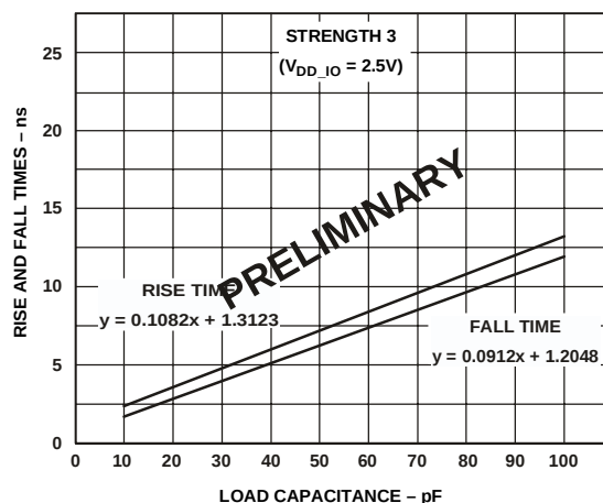
Figure 37. Typical Output Rise and Fall Time (10%–90%, V_{DD\_IO} = 2.5\text{ V} ) vs. Load Capacitance at Strength 3
