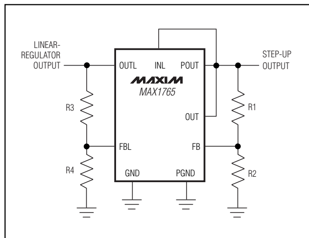
Figure 7. Feedback Connections
