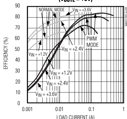
TRACK MODE EFFICIENCY vs. LOAD CURRENT ( V_{OUTL} = +5V )
