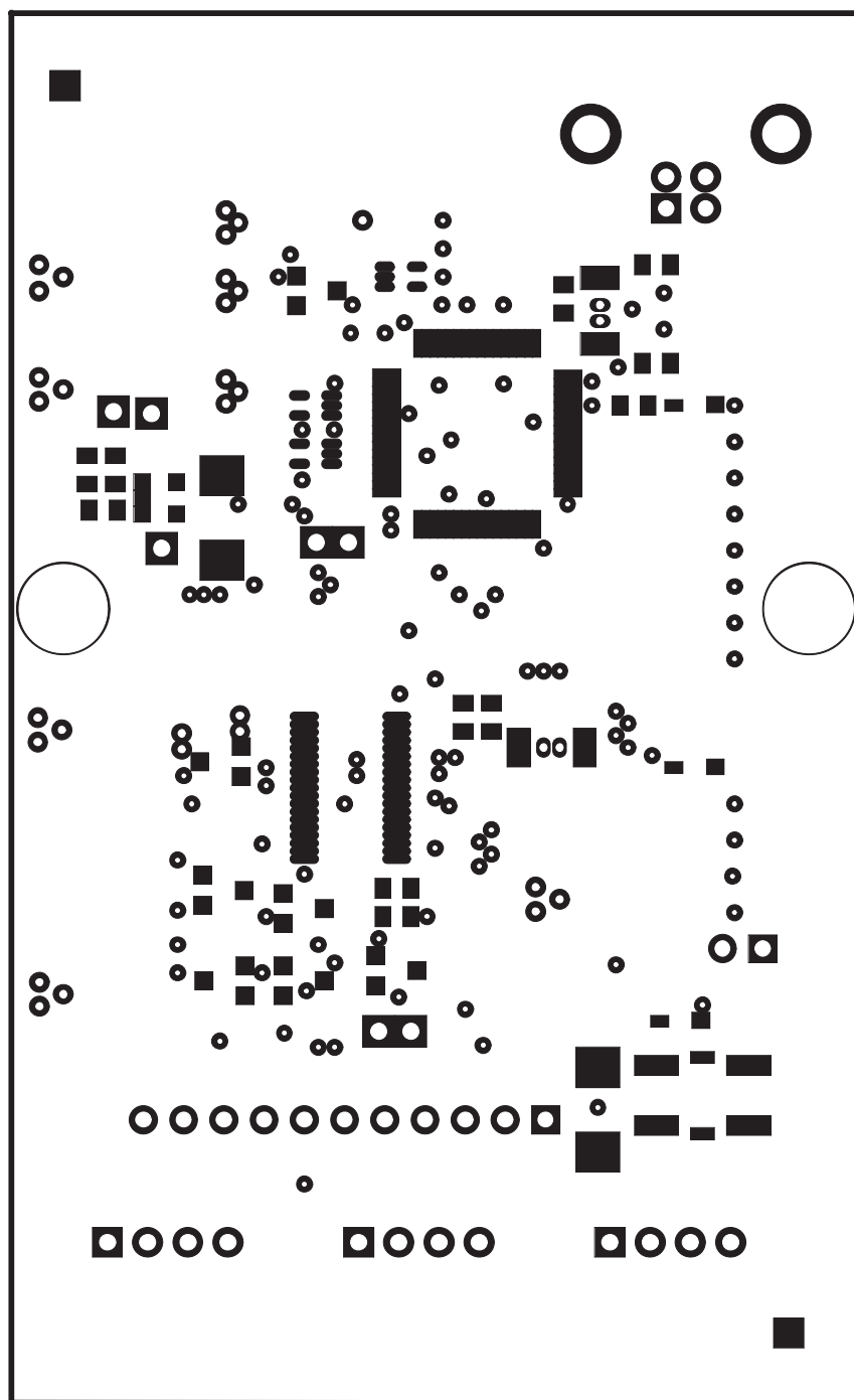
Figure 2. Solder Mask 1
