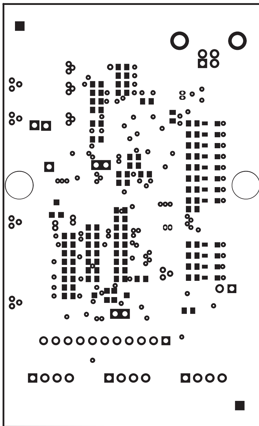
Figure 3. Solder Mask 2
