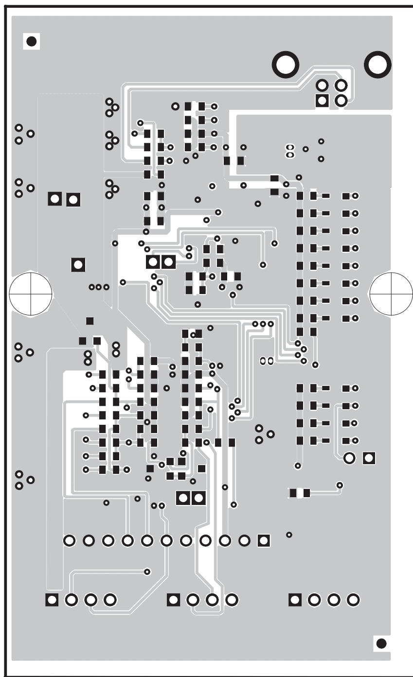
Figure 4. Board Layer 2
