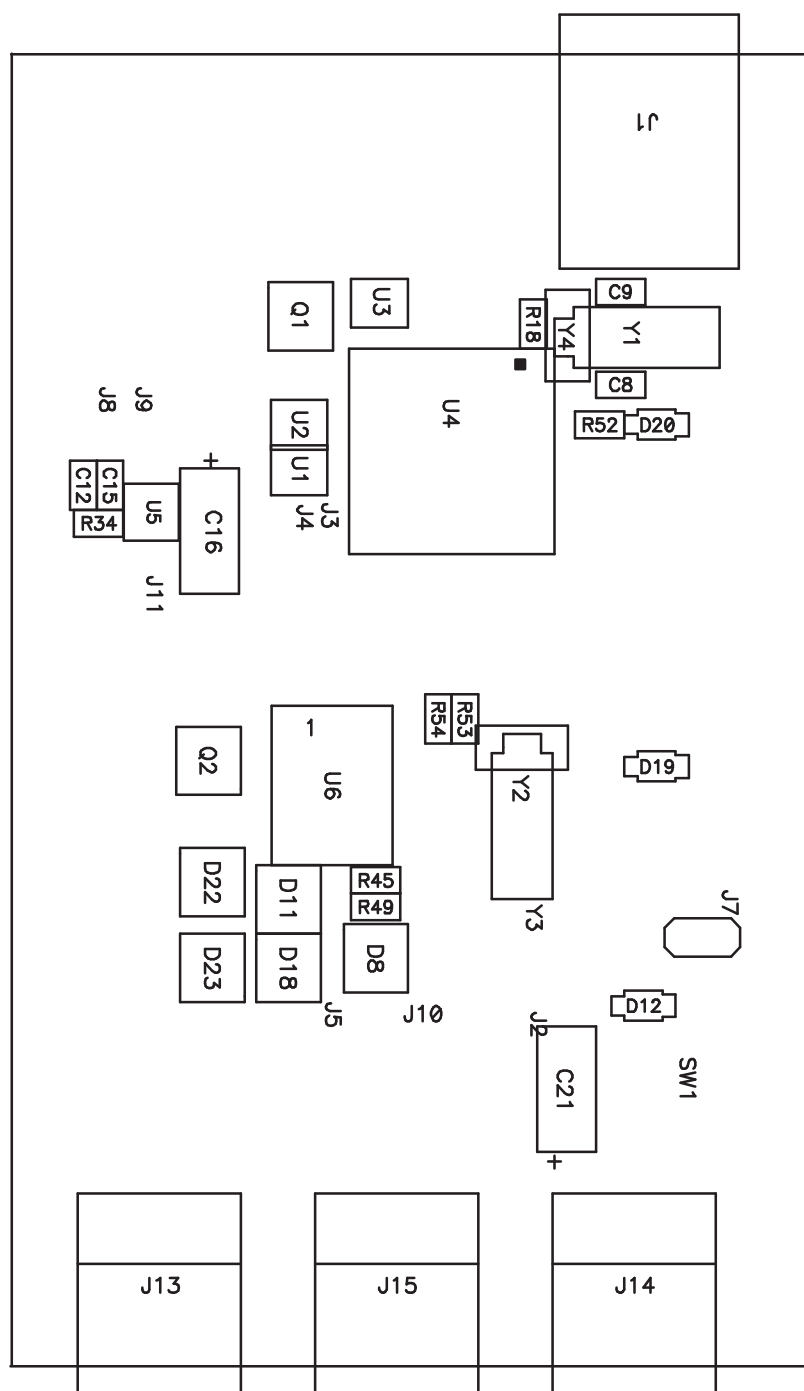
Figure 5. Component Placement 1
