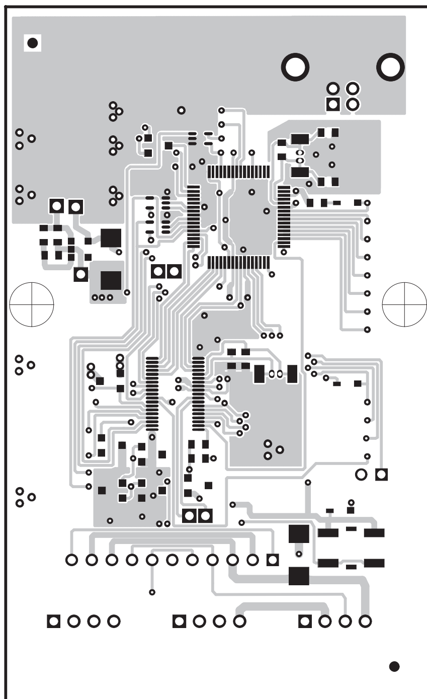
Figure 1. Board Layer 1
