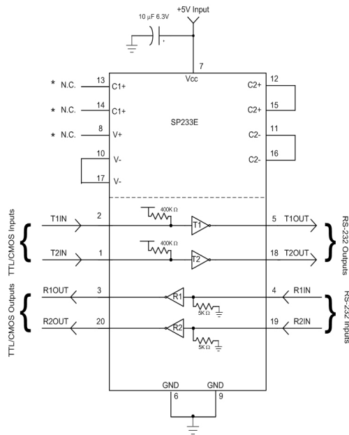
Figure 9, SP233ECT Typical Application circuit
