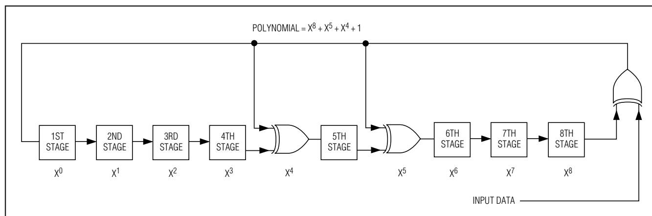
Figure 5. CRC Polynomial
