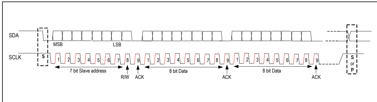
Figure 22. I 2 C Bus Protocol
