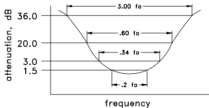
BANDPASS, ELLIPTICAL TYPICAL FREQUENCY RESPONSE
