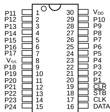
NJU3719AM
