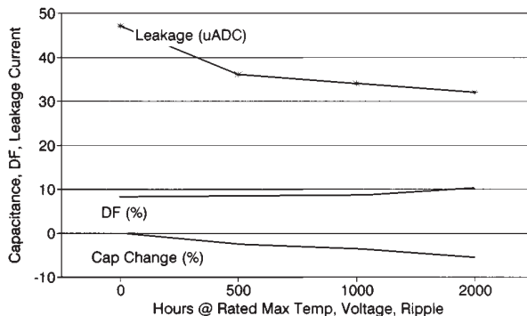
Life Test Data 380LX222M100J042 Capacitance, DF, Leakage Current
