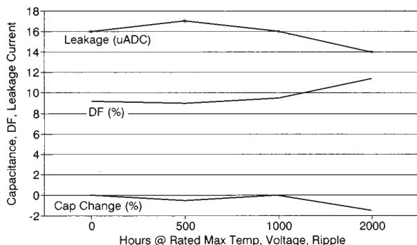
Life Test Data 380L222M050K012 Capacitance, DF, Leakage Current
