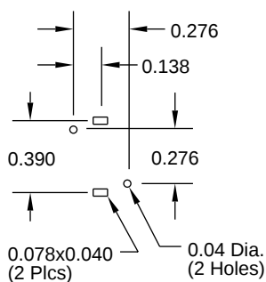
Pad Layout
