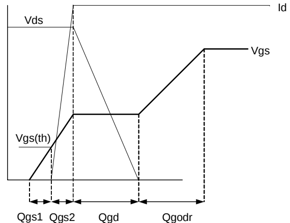
Fig 16b. Gate Charge Waveform
