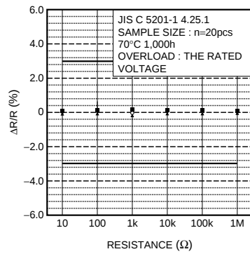
Fig.8 Endurance at 70^\circ\text{C}
