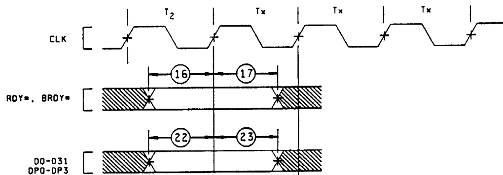
FIGURE 5. Timing waveforms.
