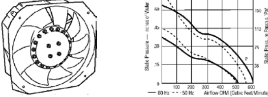
Mounting: From either face using four .177" (4.5 mm) holes. Weight: 42 oz. (1200 g). Housing: Aluminum. Capacitor: Included; mounted on unit within envelope. Bearings: Double-shielded ball. Options: Grill guard #78128-2-4039. Dimensions: 8.86" x 8.86" x 3.15". AC Fan. Ball bearing, all metal, air exhaust — over struts. Terminal block.
