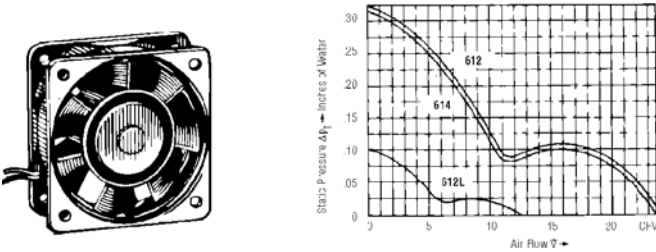
Fan of fiberglass reinforced plastic. PBTP housing, PA impeller. Electronically commutated DC motor. Clockwise rotation viewed from rotor, air output over struts. Elec. connection via 2 leads AWG 22, TR 64, 12 in. (310 mm). Mass: 3 oz. (85 g). Ball bearing. Dimensions: 2.44" x 2.44" x 1.0" (60 mm x 60 mm x 25 mm).
