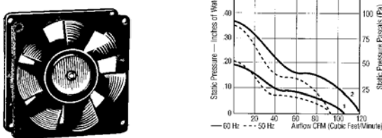
Housing is metal with plastic impellers. Connection terminates with two flat pins, .118" x .02". Air exhaust — over struts. Mounting is either face using four .169" (4.3 mm) holes. Dimensions: 5.00" x 5.00" x 1.50" (127 mm x 127 mm x 38 mm).
