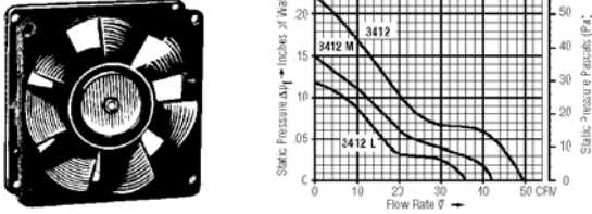
Fan of fiberglass reinforced plastic. PBTP housing, PA impeller. Electronically commutated external rotor DC motor. Clockwise rotation viewed from rotor, air output over struts. Elec. connection via 2 leads AWG 22, TR 64, 12 in. (310 mm). Mass: 150 g. Dimensions: 3.62" x 3.62" x 1.26" (119 mm x 119 mm x 32 mm).
