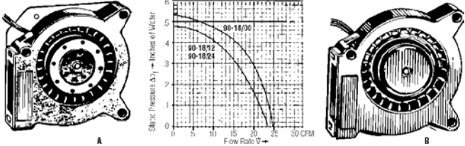
Fig. A. Model RL90-18/00 Blower Housing of fiberglass reinforced plastic (PC) and metal plate, impeller of fiberglass reinforced plastic (PA). Shaded pole motor. Clockwise rotation viewed from rotor, air output through housing window. Elec. connection via 2 leads AWG 18, TR 64, 12 in. (310 mm). Mass: 24.5 oz. (680 g). Dimensions: 4.75" x 4.75" x 1.45" (121 mm x 121 mm x 37 mm).
