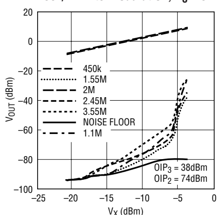
450k/2M Intermodulation, V_S = 5\text{V}
