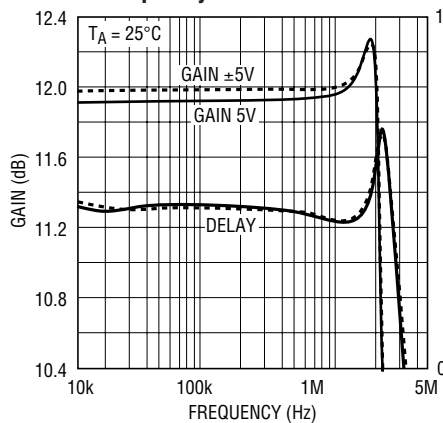
Passband Gain and Delay vs Frequency
