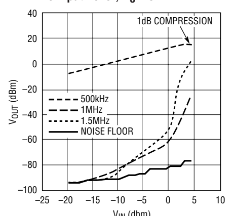
500kHz Distortion vs Input Level, V_S = 5\text{V}
