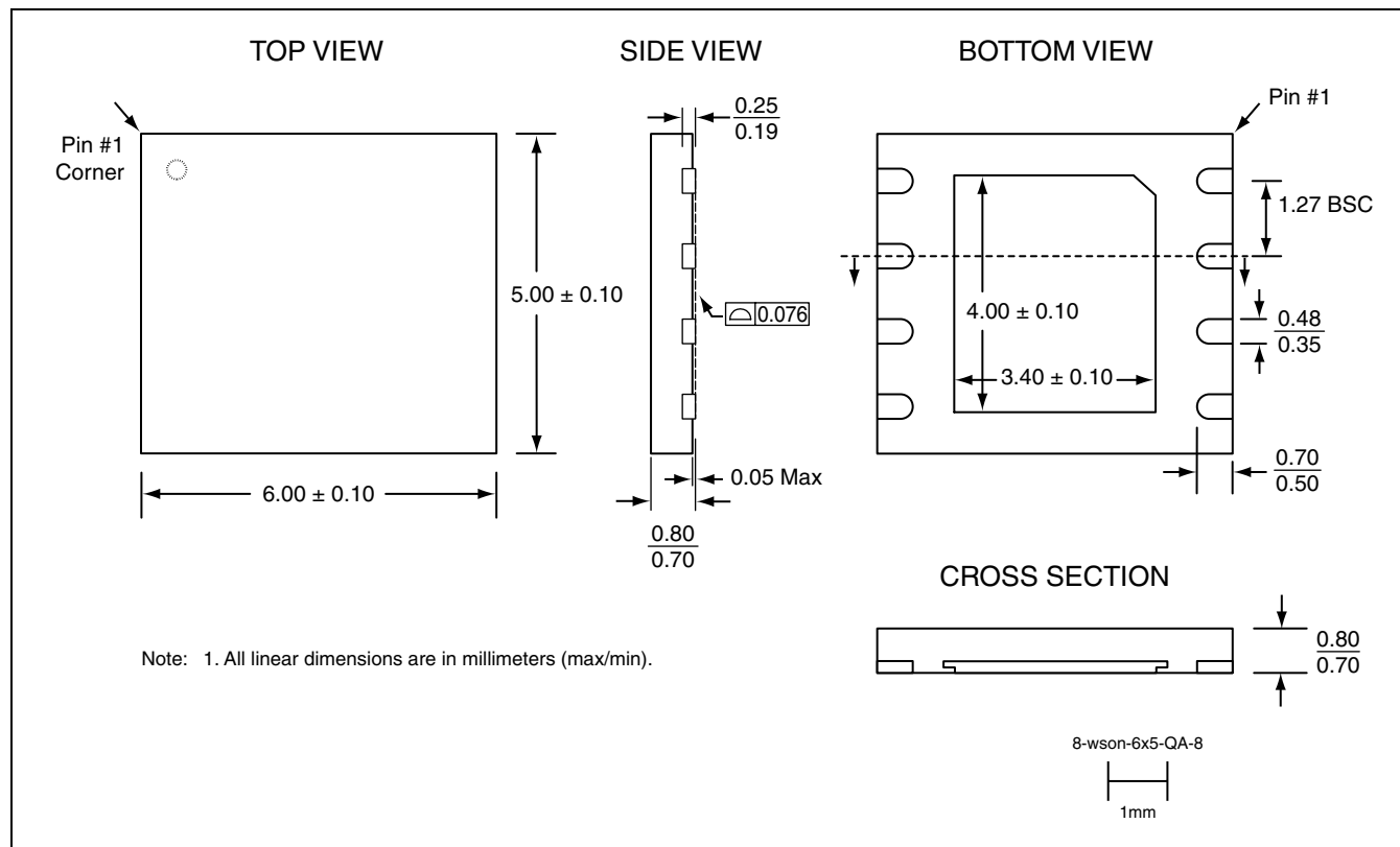
8-CONTACT VERY-VERY-THIN SMALL OUTLINE NO-LEAD (WSN) SST PACKAGE CODE: QA
