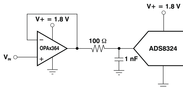
Figure 26. OPAx364 Directly Drives the ADS8324
