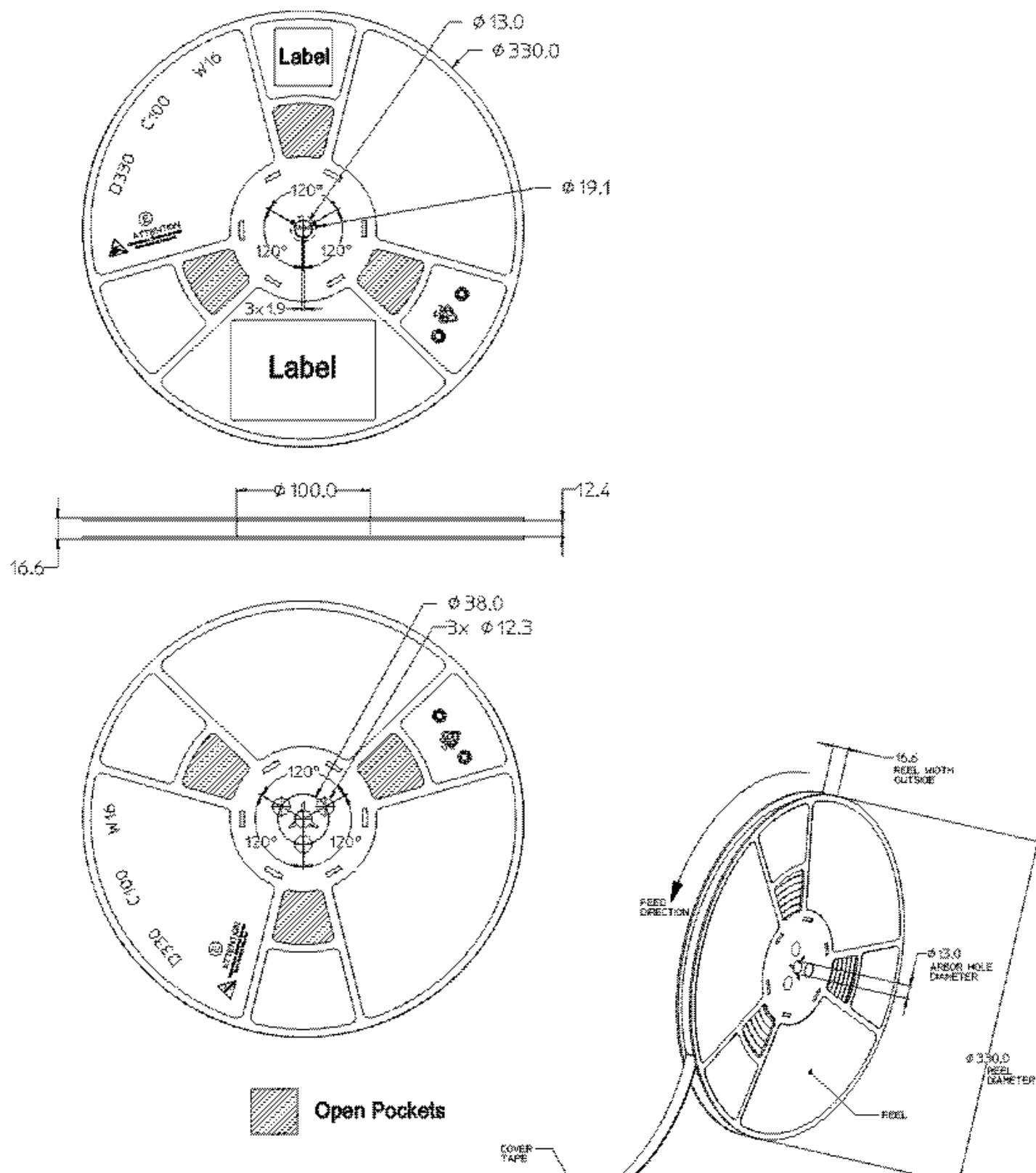
Figure 21. Emitter reel packaging.
