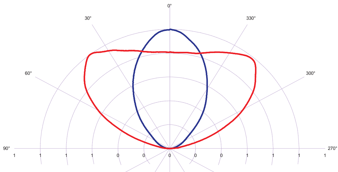
Figure 17. Typical polar radiation pattern for green and royal-blue lambertian.
