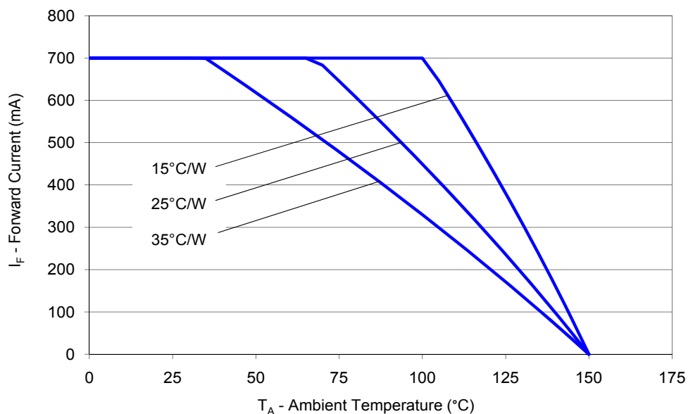
Figure 13. Maximum forward current vs. ambient temperature, based on T_{J\text{MAX}} = 150^{\circ}\text{C} .
