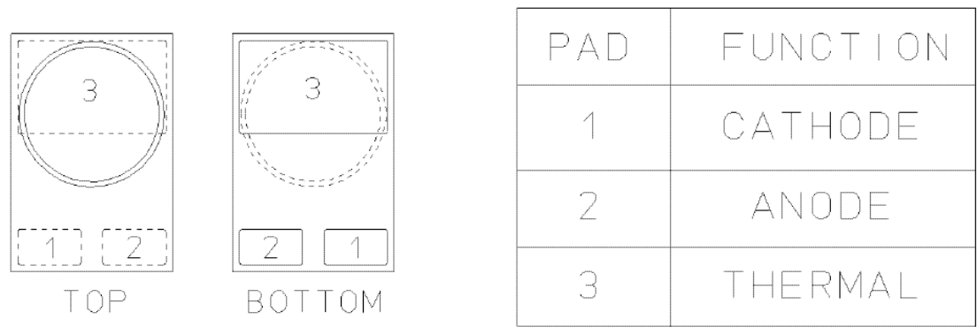
Figure 2. Pad configuration.
