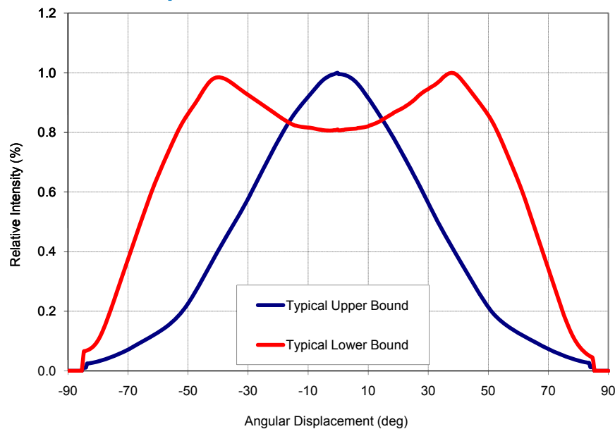
Figure 16. Typical representative spatial radiation pattern for green and royal-blue lambertian.
