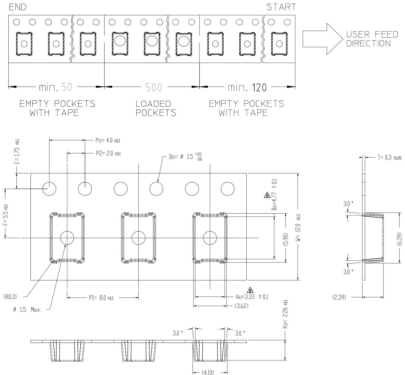
Figure 20. Emitter pocket tape packaging.
