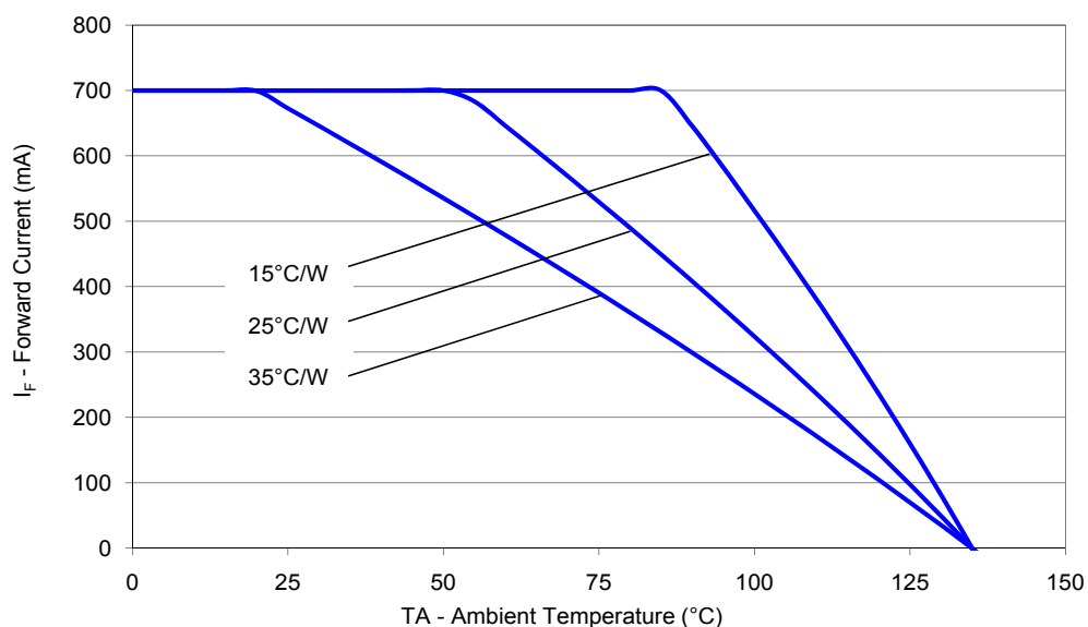
Figure 14. Maximum forward current vs. ambient temperature, based on T_{J\text{MAX}} = 135^{\circ}\text{C} .
