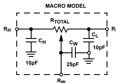
Circuit #3 SPICE Macromodel
