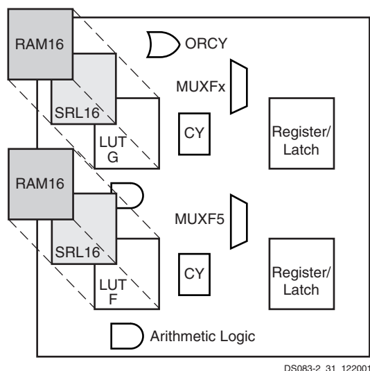
Figure 33: Virtex-II Pro Slice Configuration
