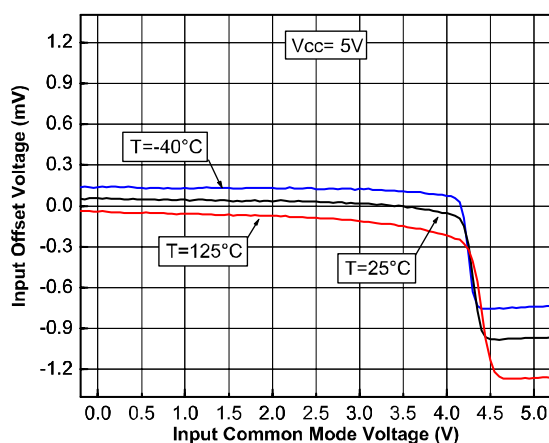
Figure 17: Input offset voltage vs input common mode voltage at V_{CC} = 5 V
