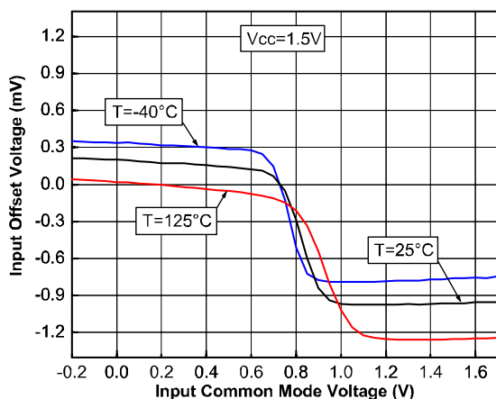
Figure 16: Input offset voltage vs input common mode voltage at V_{CC} = 1.5 V
