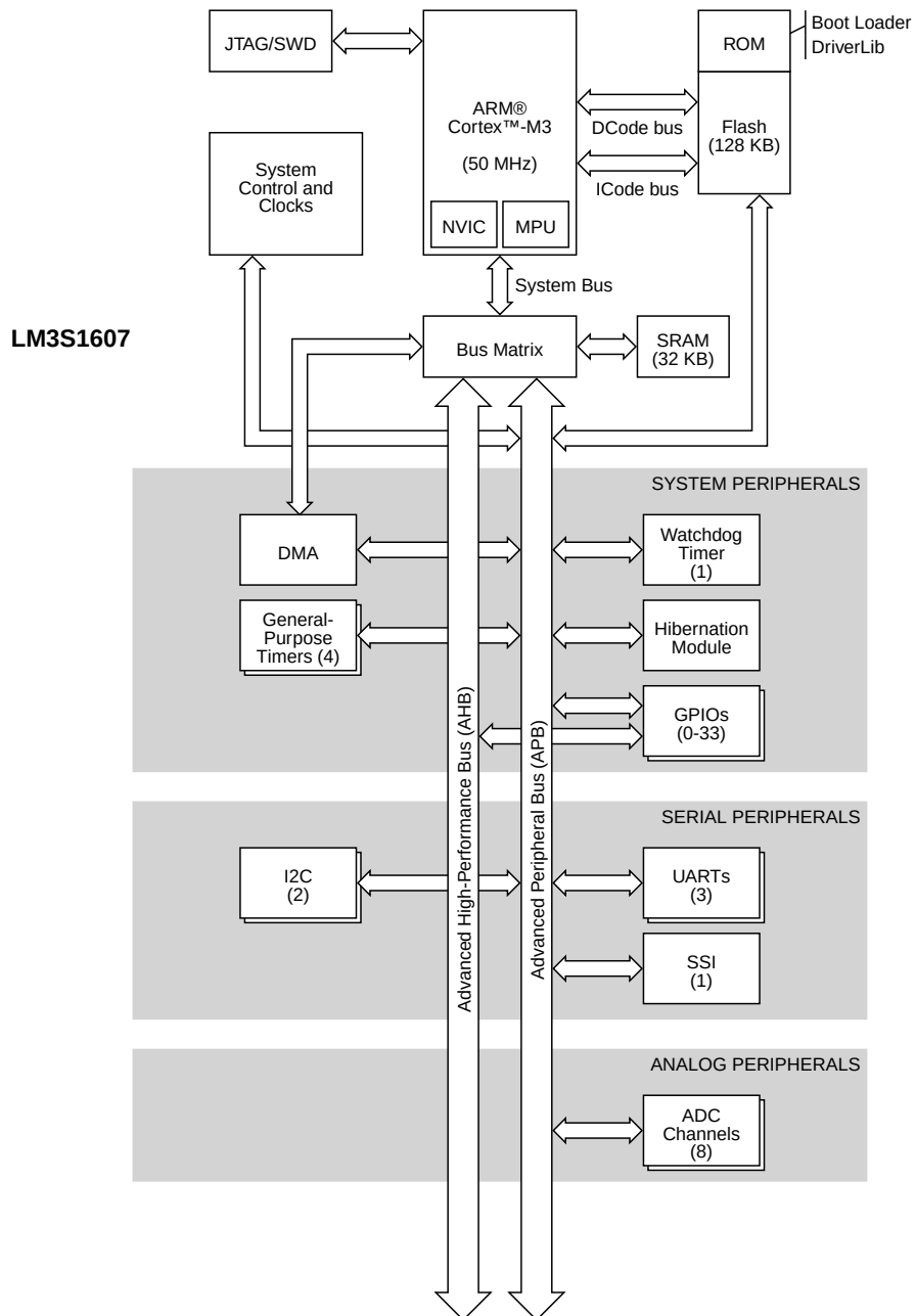
Figure 1-1. Stellaris® LM3S1607 Microcontroller High-Level Block Diagram
