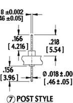
⑦ POST STYLE
