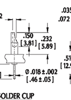
③ SOLDER CUP
