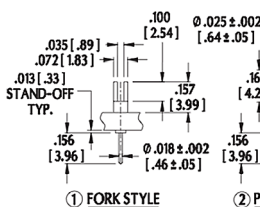
① FORK STYLE
