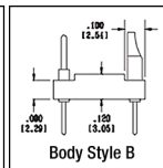
Body Style B
