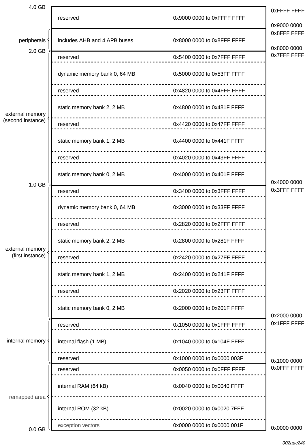
Fig 3. Memory map
