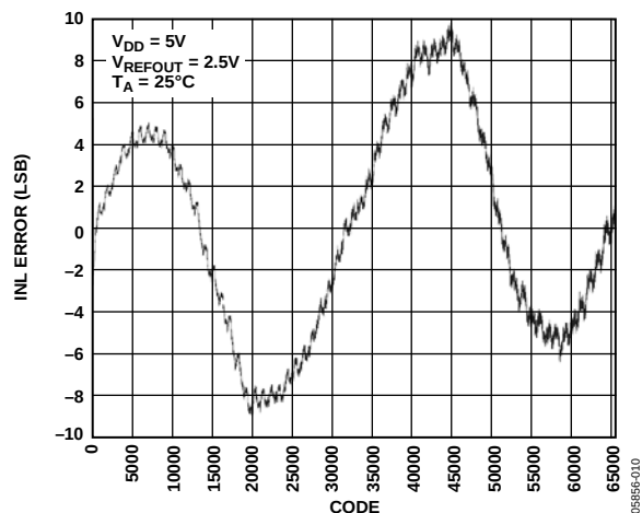
Figure 11. AD5664R-5 INL, Internal Reference
