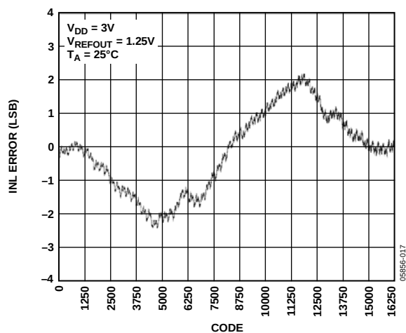
Figure 18. AD5644R-3 INL, Internal Reference
