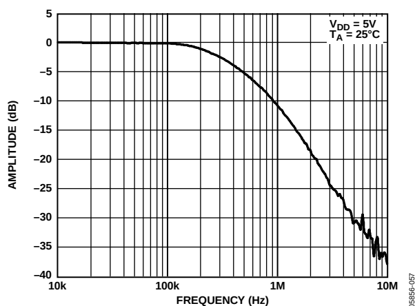
Figure 50. Multiplying Bandwidth
