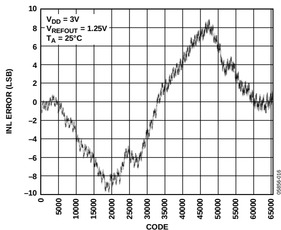
Figure 17. AD5664R-3 INL, Internal Reference
