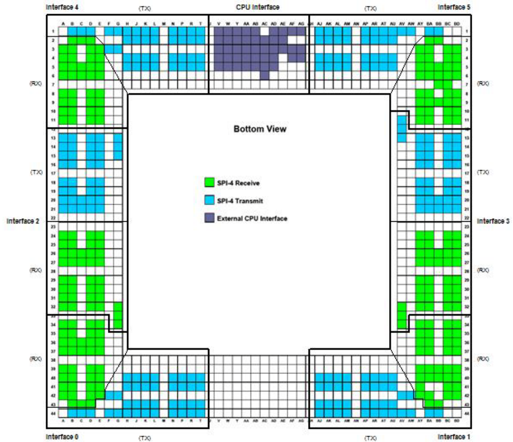
Figure 11. Interface Mapping
