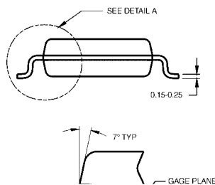
14-Lead Small Outline Package (SOP), EIAJ TYPE II, 5.3mm Wide Package Number M14D
