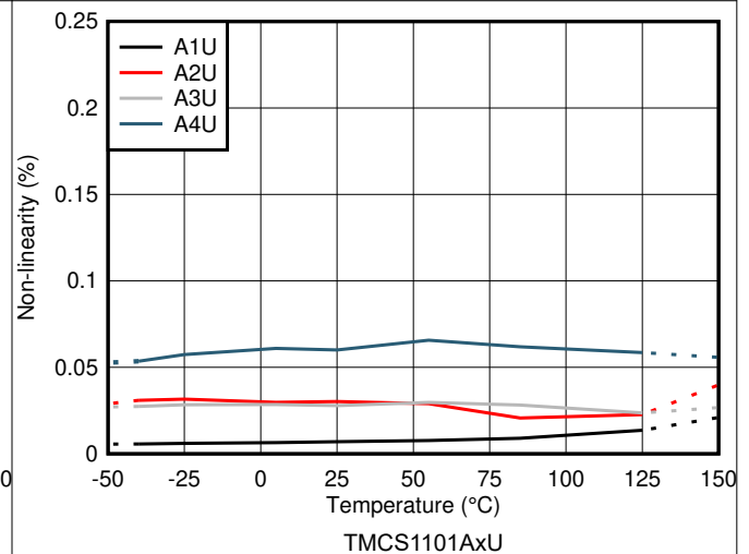
Figure 6-6. Non-Linearity vs Temperature
