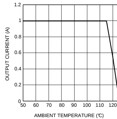
Figure 38. Thermal Derating Curve
