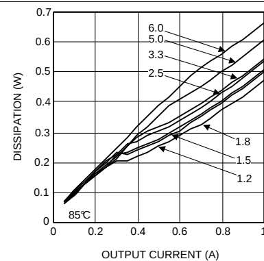
Figure 22. Dissipation 12-V Input at 85°C
