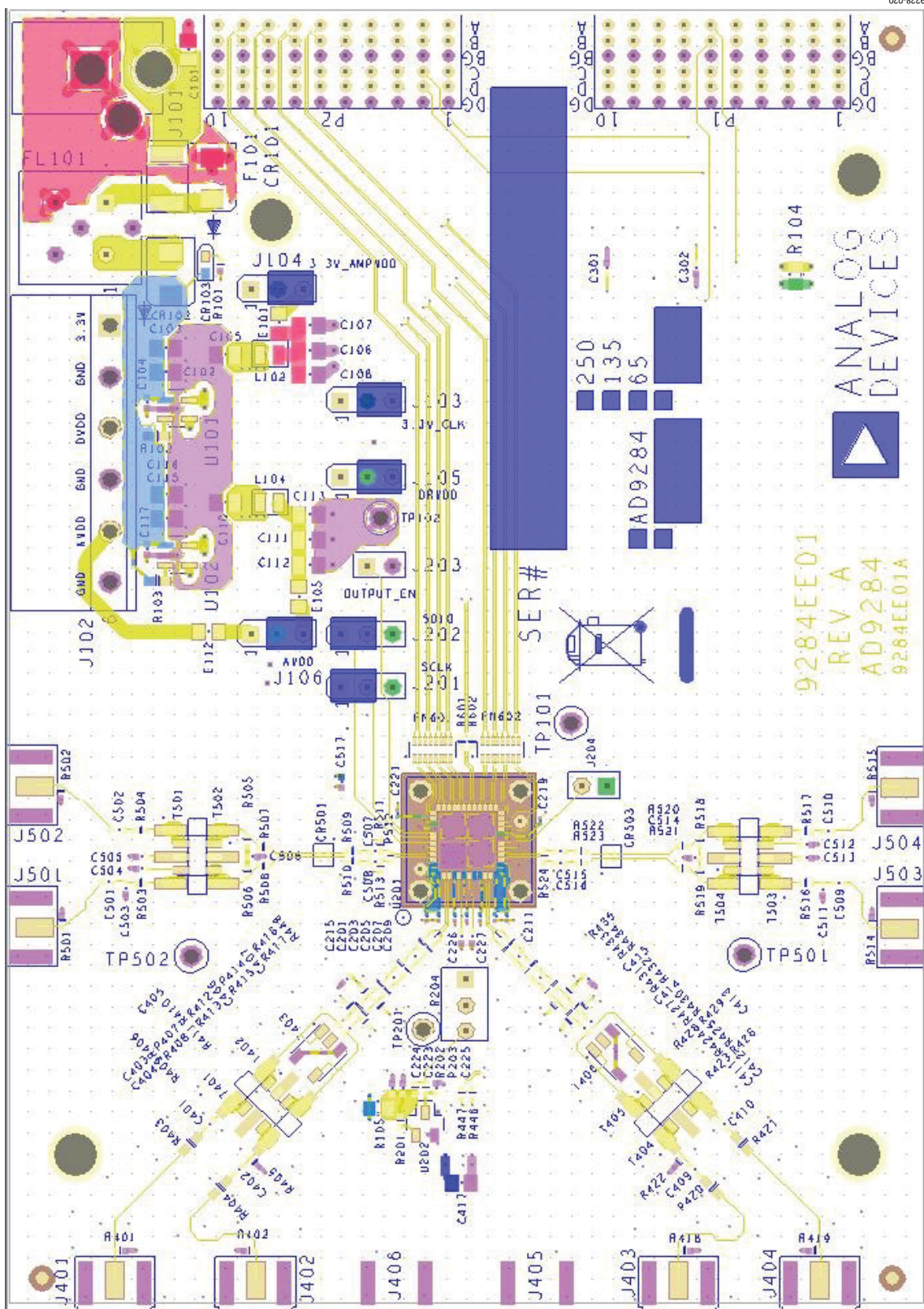
Figure 20. Top Side
