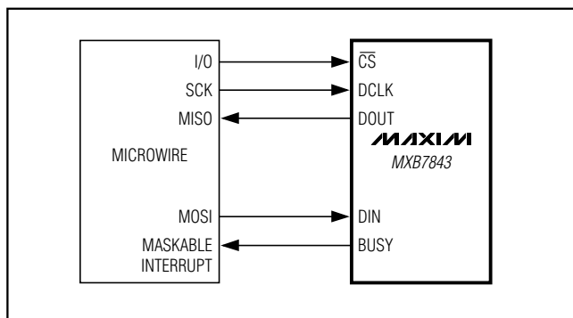
Figure 11. MICROWIRE Interface
