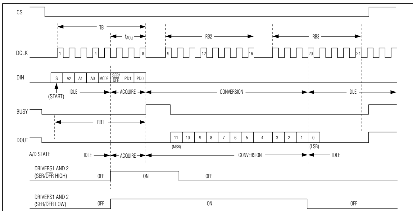
Figure 7. Conversion Timing, 24-Clock per Conversion, 8-Bit Bus Interface
