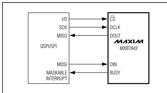
Figure 12. QSPI/SPI Interface
